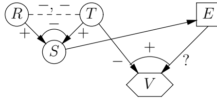
Figure 4: The qualitative Sore Throat diagram.
