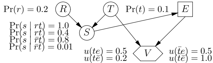
Figure 2: The Sore Throat influence diagram.
