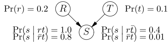
Figure 1: The Sore Throat belief network.
