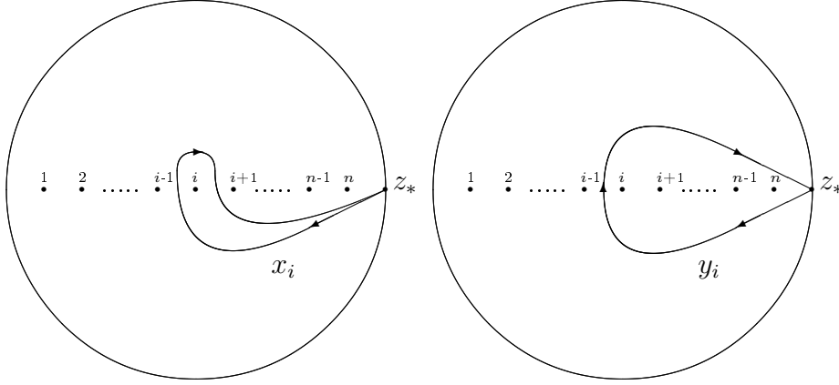
FIGURE 1.1: PATHS REPRESENTING THE GENERATORS x_i AND y_i OF \pi_1(D_n, z_*) .
