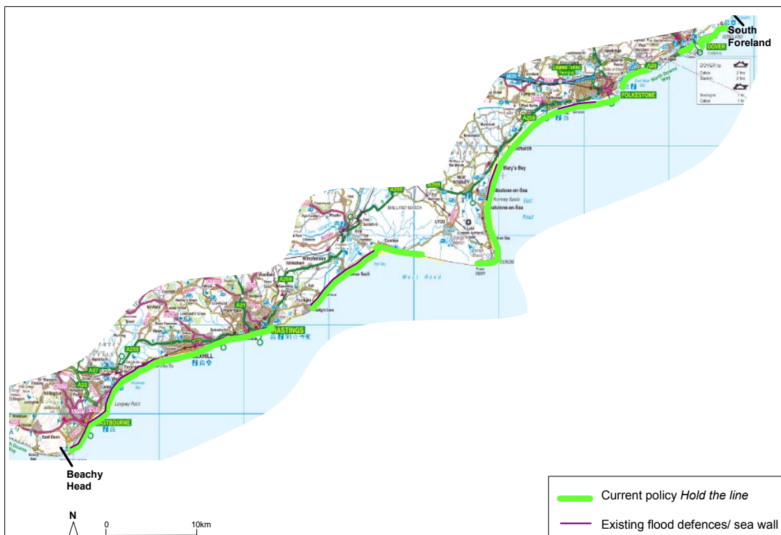
Figure 11.3 South Foreland - Beachy Head: Current shoreline position and management policy
