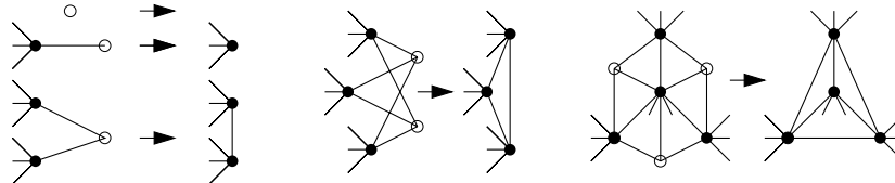
Fig. 5. The Six Reduction Rules for Treewidth Three
