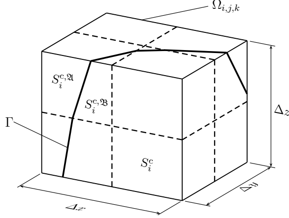
Figure 10. Piecewise linear representation of the intersections between the boundary of control volume \Omega_{i,j,k} and the interface \Gamma . The parts of the surface bounded by the dashed lines are the inner faces of cells around node (i, j, k) as shows in Figure 3.
