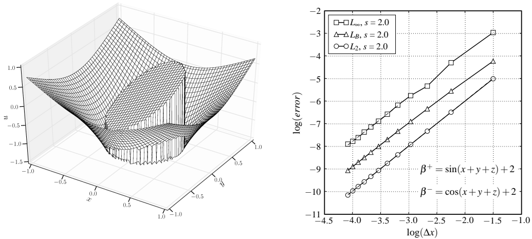
Figure 11. Solution for example 1 at z = 0 (left) and convergence results (right). The slope s of the linear least square fit is the order of convergence.
