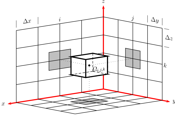
Figure 2. Control volume \Omega_{i,j,k} . Discrete solution values are located at grid nodes i, j, k .
