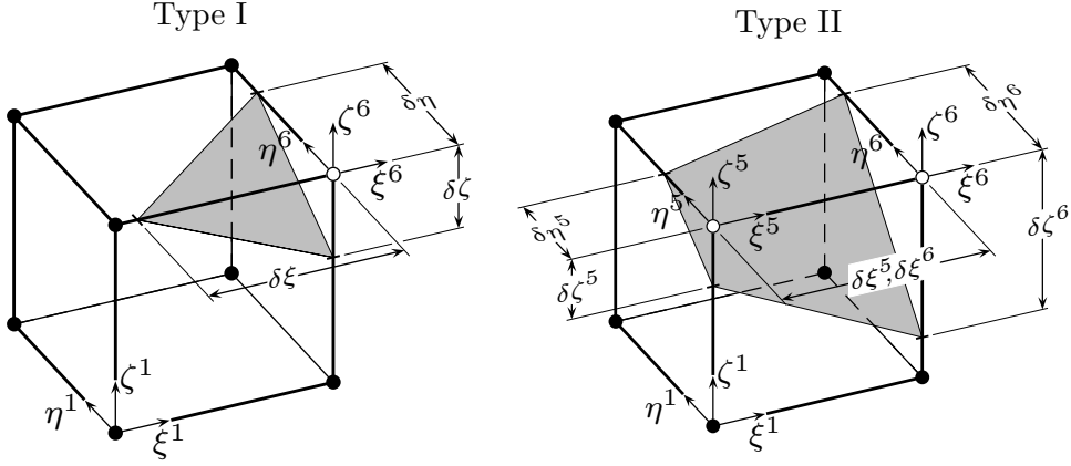
Figure 8. Coordinate systems and naming conventions for the two-term asymptotic solution approach. The pictures show exemplary configurations for a cut-cell of type I with \mathbf{n} = 6 on the left, and \mathbf{n}_1 = 5, \mathbf{n}_2 = 6 for a type II cut-cell on the right.
