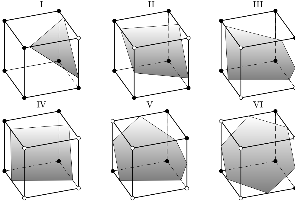
Figure 4. Different types of cut-cells considered in this work. Nodes marked with \circ and \bullet respectively, are on the same side of the interface.
