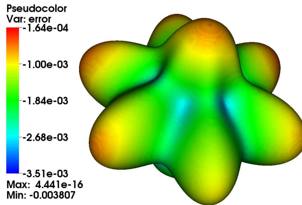
Figure 14. Surface error plot of the star like interface of example 3.
