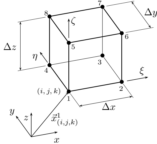
Figure 6. Node numbering and local coordinate system for a computational cell (i, j, k) . For normal cells and non-singular cut-cells the origin of the local coordinate system used for the trilinear solution ansatz is always at node number 1.
