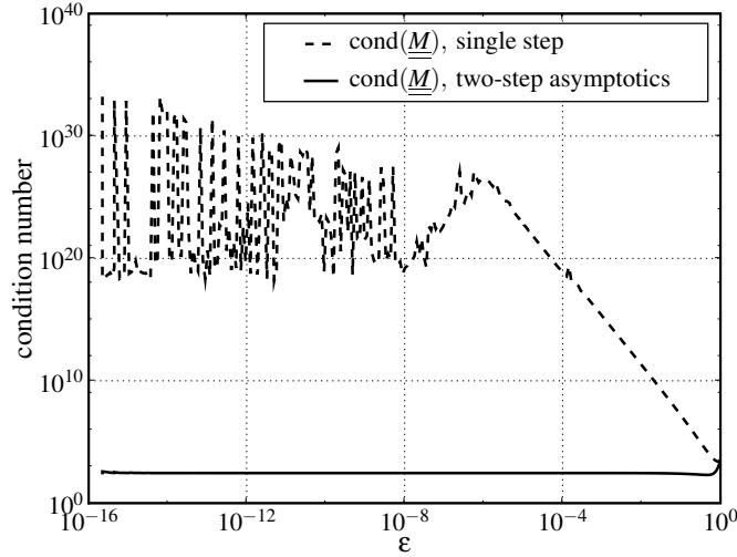
Figure 9. Condition number of the minimization matrix \underline{M} according to (25) and (53) for a singular cut-cell of type I with \beta^+ = \beta^- = 1 and \varepsilon = \delta\xi = \delta\eta = \delta\zeta .
