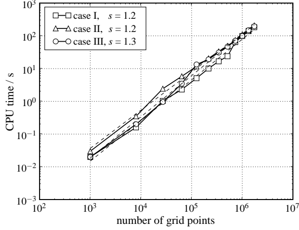
Figure 16. CPU times for solving the resulting set of linear equations as a function of the total number of grid points and different ratios of the coefficient \beta . The scaling factors s has been evaluated using a linear least square fit.
