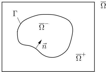
Figure 1. Domain \overline{\Omega} with sub-domains \overline{\Omega}^+ , \overline{\Omega}^- , and embedded interface \Gamma .
