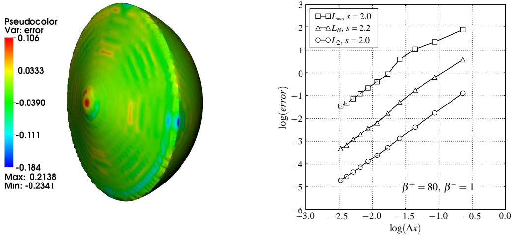
Figure 17. Error at the interface and convergence results for the oak acorn (example 4). The surface error plot has been obtained on a grid with 100 \times 100 \times 100 points. The scaling factors s has been evaluated using a linear least square fit.
