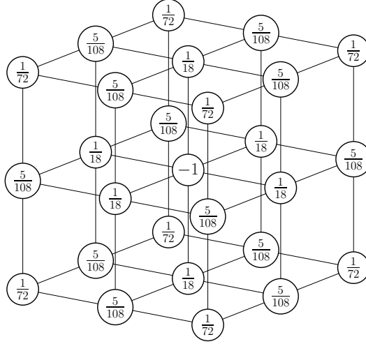
Figure 7. Stencil elements for a control volume with \beta = 1 , \Delta x = \Delta y = \Delta z = 1 where all adjacent cells are normal cells not cut by an interface.
