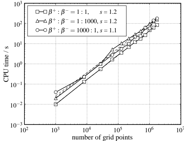
Figure 13. CPU times for solving the resulting set of linear equations of example 2 as a function of the total number of grid points and the ratio of the coefficient \beta^+ : \beta^- . The scaling factors s has been evaluated using a linear least square fit.
