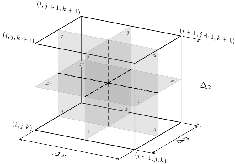
Figure 3. Cell C_{i,j,k} with node indices. The grey shaded internal faces with indices 1–12 are surface parts of the control volumes having a partial volume within the cell. The eight cuboids formed by the internal faces of the cell with edge lengths \Delta x/2 , \Delta y/2 , and \Delta z/2 belong to different control volumes and are called sub-cells.
