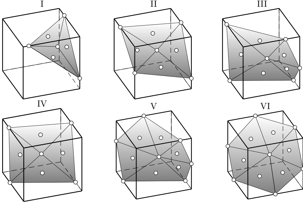
Figure 5. Interface discretisation by triangulation for the different types of cut-cells. Discrete jump conditions are applied at the triangle corner points and the triangle barycenters which are marked with circles.
