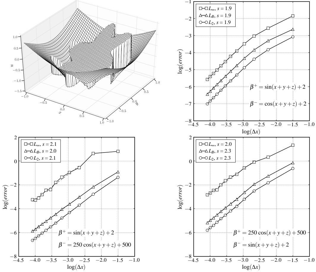
Figure 15. Solution for example 3 at z = 0.2 and convergence results for different \beta -ratios for the star-example. The scaling factors s has been evaluated using a linear least square fit.
