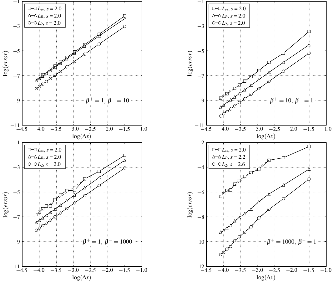
Figure 12. Convergence results for example 2 with a spherical interface and different ratios of the coefficients \beta^+ : \beta^- . The slope s of the linear least square fit is the order of convergence.
