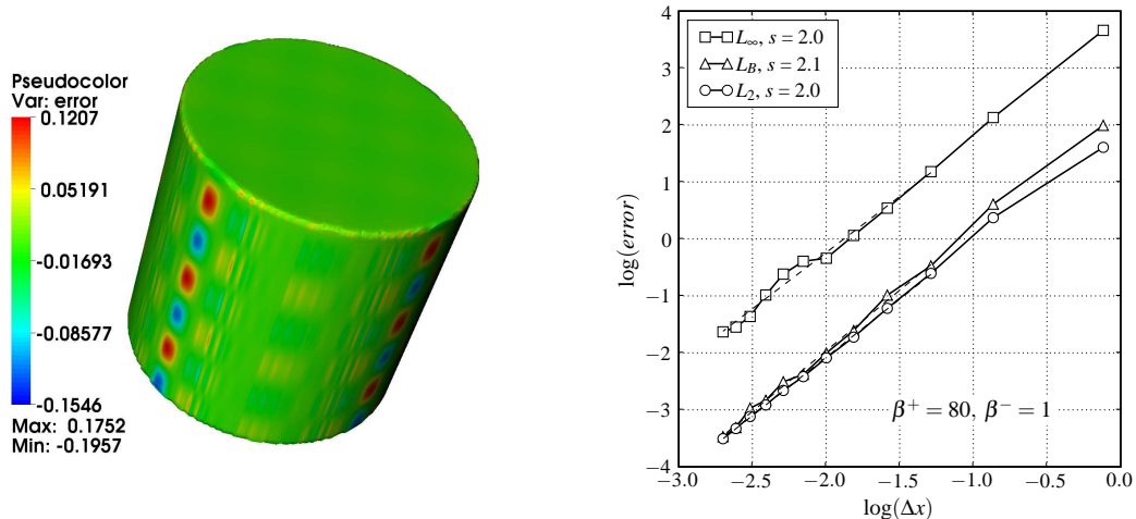
Figure 18. Surface error plot and convergence results for a cylinder interface. The scaling factors s has been evaluated using a linear least square fit.
