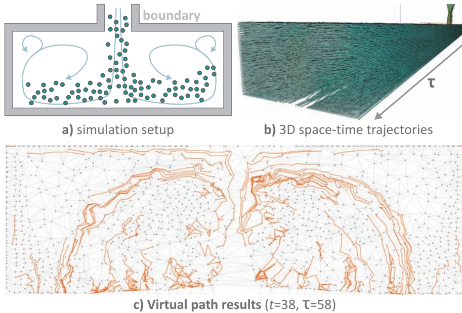
Abbildung 15: SPH Simulation: Slice of the SPH simulation at t = 38 . a) shows the simulation setup and the domain, b) a rendering of the trajectories in space time, and c) the base grid with virtual path structures (light grey, 10% longest highlighted in orange, \tau = 58 )
