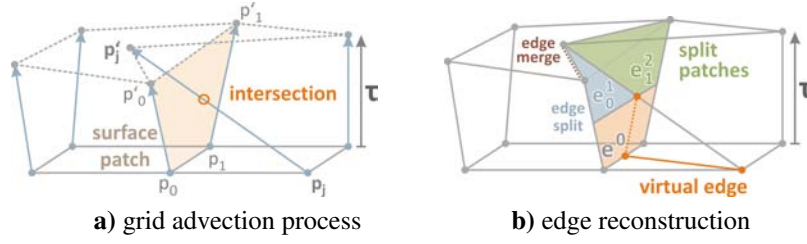
Abbildung 5: Conceptual representation of the splitting procedure: Moving edges form bilinear surface patches that are tested for intersections with moving particles (i.e., lines or rays). If an intersection occurs, the original edge is split into two edges and surface patches and creates a virtual edge .
