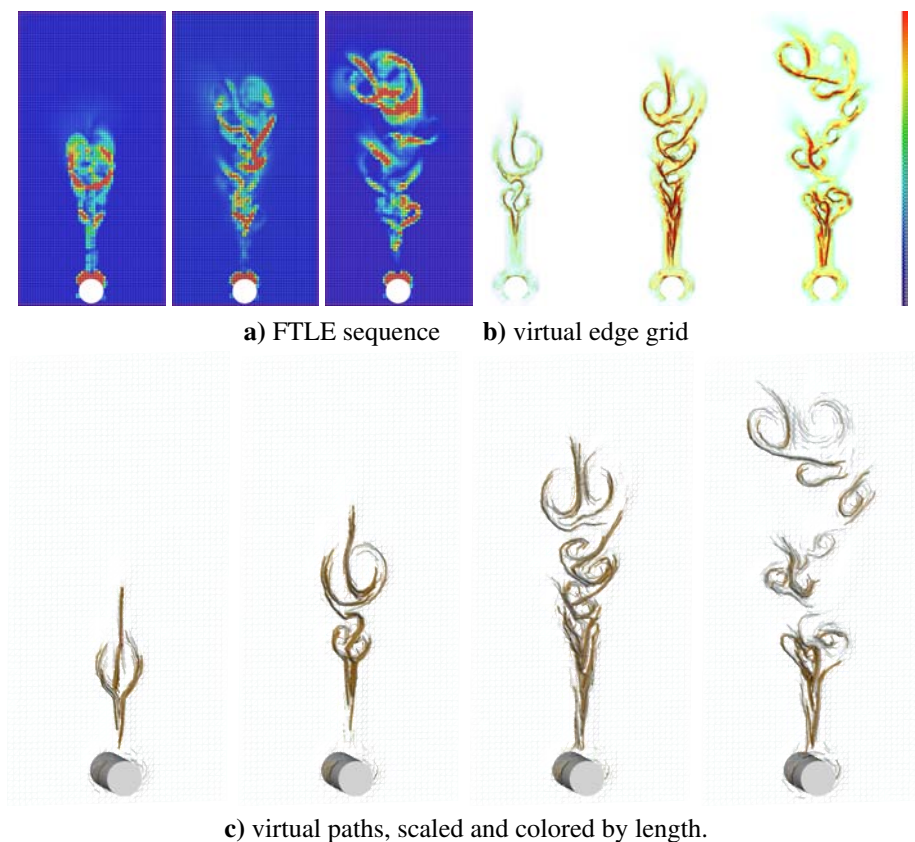
Abbildung 14: Heated Cylinder: Time sequence comparison for FTLE ( 60 \times 120 ) and triangulated virtual edge grid with 36 \times 72 and fixed \tau = 20 and t_0 = 20, 30, 40 .
