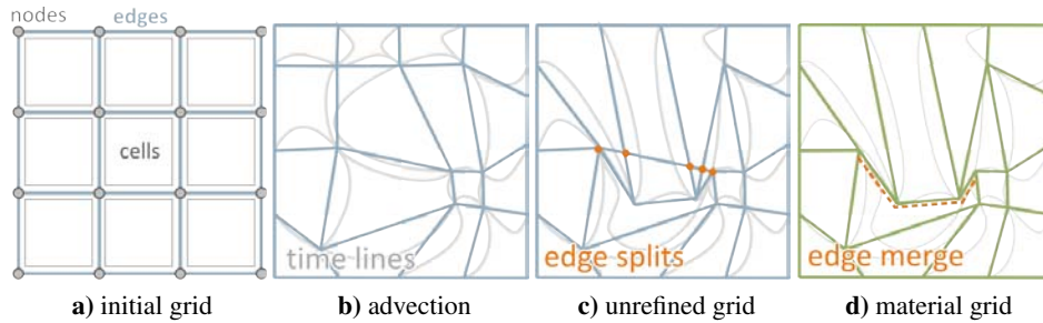
Abbildung 2: Illustration of material edges in a discrete grid to approximate the behavior of continuous time lines. The refinement of the initial grid introduces split and merge events.
