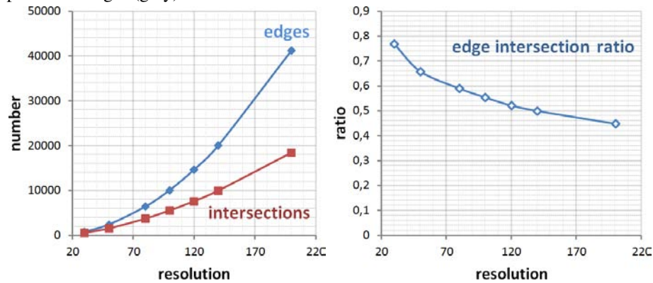
Abbildung 9: Cylinder Flow : Plot of the number of edges with increasing resolution (left) and average intersections per edge (right, c.f. Figure 17).
