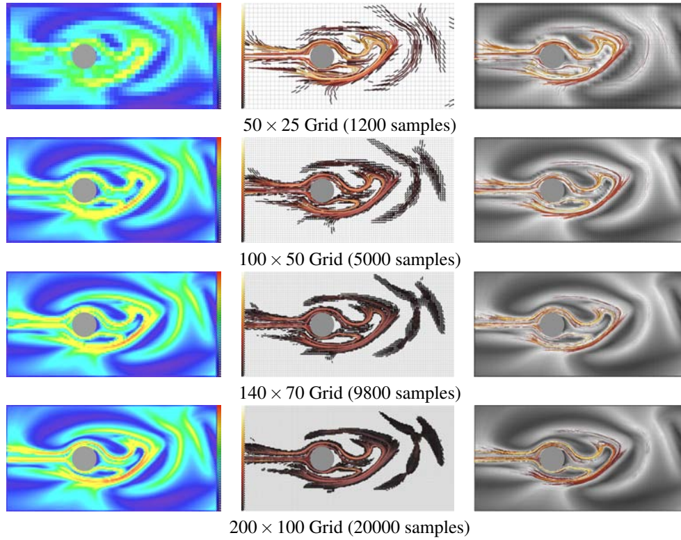
Abbildung 16: Cylinder Flow : Comparison of FTLE [Hal01a] (left column), virtual paths (center, colored by length), and overlay of both (right column, colored and scaled by length) at increasing sampling resolutions for t_0 = 0, \tau = 40 .
