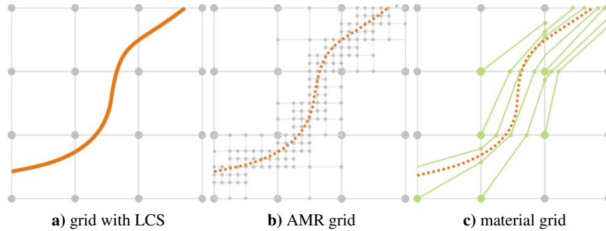
Abbildung 1: Representation of material flow structures a) in different grids: b) an AMR uses additional samples [SP07], c) our method creates intersecting edges.
