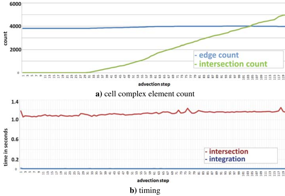
Abbildung 10: Double Gyre . Figure a) shows the number of edges in the material grid and number of intersection events, b) shows the time required for intersection and integration for each time step for the 64 \times 32 grid shown in Figure 11.
