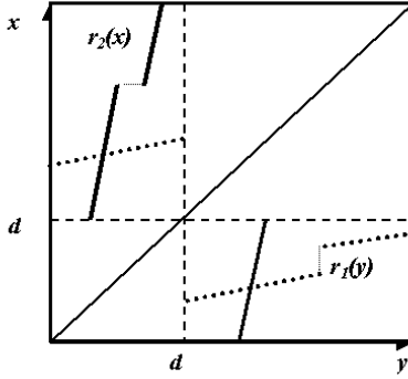
Figure 3: Reaction curves are partially increasing, but possess a unique jump down, which precludes any symmetric equilibrium.
