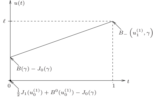
Figure 3: An intuitive picture of the location of boundary layers for a crack in 0.
