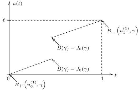
Figure 4: An intuitive picture of the location of boundary layers for a crack in the interior.
