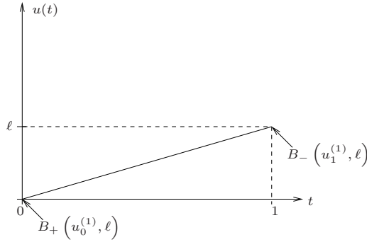
Figure 2: An intuitive picture of the location of boundary layers for \ell \leq \gamma .
