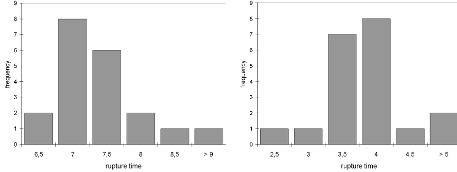
Figure 5: Statistics of first-rupture time for white noise driven thin-film flow ( l_c = 0 ): Computation of 20 sample paths for T = 5 \cdot 10^{-5} (left, mean value and standard deviation are (\mu, \sigma) = (7.1, 0.4) ) and T = 1.25 \cdot 10^{-3} (right, (\mu, \sigma) = (3.6, 0.4) ) respectively. Discretization with a = 2^{-8}L , \tau = a^2 .
