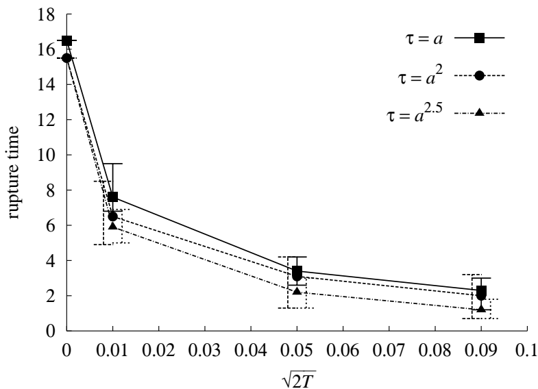
Figure 6: Monitoring the scheme for white noise driven thin-film flow ( l_c = 0 ): Mean rupture time (averaged over six sample paths each) as a function of various noise intensities \sqrt{2T} for several time discretizations. Errorbars indicate the standard deviation. For \tau = a^2 and \tau = a^{2.5} errorbars were shifted to the left and right by 0.002, respectively, for better visibility. Spatial discretization a = 2^{-9}L . All runs were started with same initial data.
