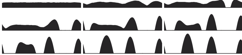
Figure 3: Snapshots at times t = 0.025, 2.9, 3.0, 3.1, 3.2, 3.3, 3.4, 3.5, 4.0 for the stochastic TFE with correlation length l_c = 0 and noise strength T = 0.00125 . The discretisation parameters, initial conditions and spatial domain size are the same as in Figure 2.
