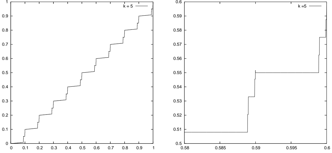
Figure 1: Graph of the function \psi from (2.4) on the interval [0, 1] (left) and a zoom into a smaller interval (right), computed for the values of the set \mathcal{D}_5 , \gamma = 10 and n = 2 . One can clearly see the non-monotonicity and discontinuity near the value x = 0.59 (right).
