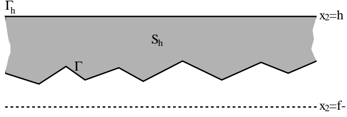
Figure 1: Geometrical setting of the scattering problem.
