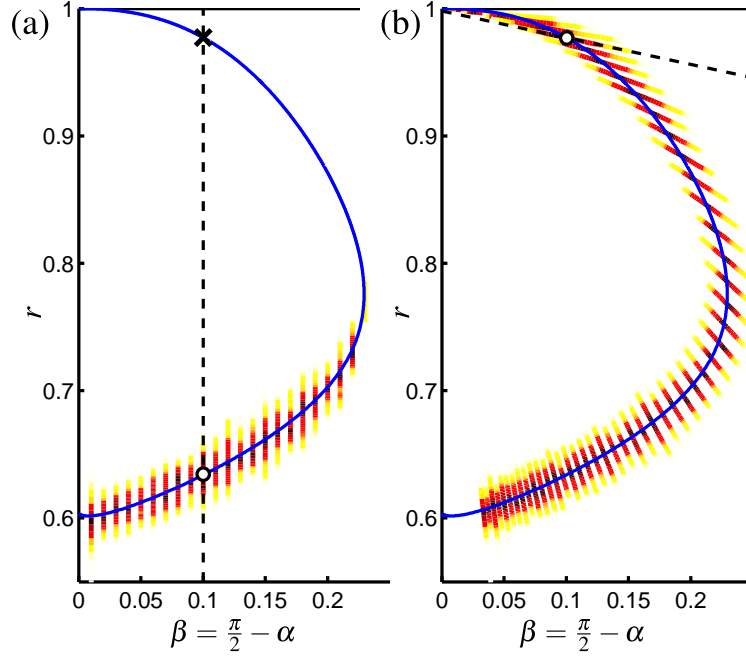
Figure 2: Chimera states projected to the (\beta, r) plane ( N = 400 , A = 0.9 ). Panel (a): Uncontrolled chimeras; sequence of simulation runs with stepwise increasing parameter \beta . Panel (b): Controlled chimeras; sequence of simulation runs with stepwise increasing control gain K . Blue curve: numerically computed chimera solution of the continuum limit equation (3). Color/shade patterns: observed density in each run (darker=higher density, see also histograms in Fig. 3). Highlighted runs along dashed lines correspond to the parameter values used in Fig. 1 and Fig. 3.
