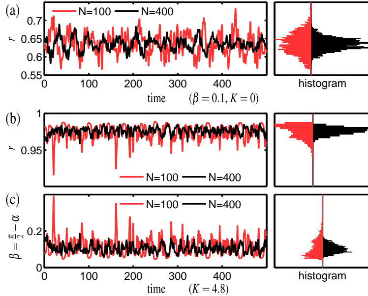
Figure 3: Time profiles and histograms of global order parameter r for chimera without control (a), and r and \beta for chimera with feedback control (b) and (c), for N = 100 and N = 400 oscillators ( K = 4.8 for (b,c), A = 0.9 ).
