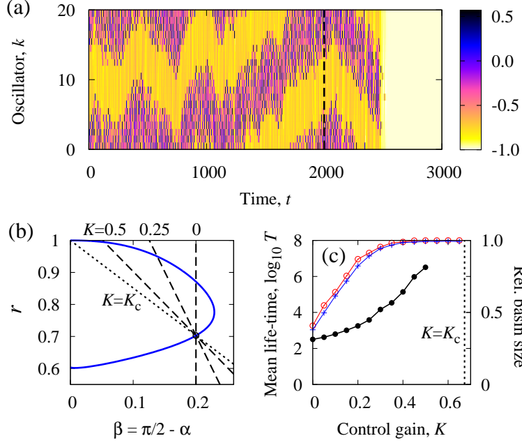
Figure 4: Influence of the control on a stable chimera state. Panel (a): Switching of the control with K = 1 at t = 2000 permits the subsequently observed collapse for N = 20 . Panel (b): Controlling the same chimera state with increasing values of the control gain K . Panel (c): mean life-time before collapse for N = 20 (dots); fraction of random initial conditions attracted by the chimera state for N = 20 (circles) and N = 100 (crosses)
