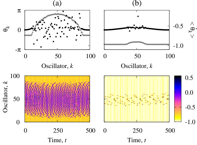
Figure 1: Chimera states far away from complete coherence (a) and close to coherence (b), obtained by numerical simulation of (1), (2) with A = 0.9 . Upper panels: Snapshot of phases (black) and time-averaged phase velocities (gray). Lower panels: Space-time plots of angular velocities. We require feedback control (6) to observe pattern (b).
