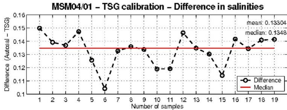
Fig. 1.9: Calibration of the thermosalinograph salinity using bottle samples from the se-water inlet at the ship's bow.
