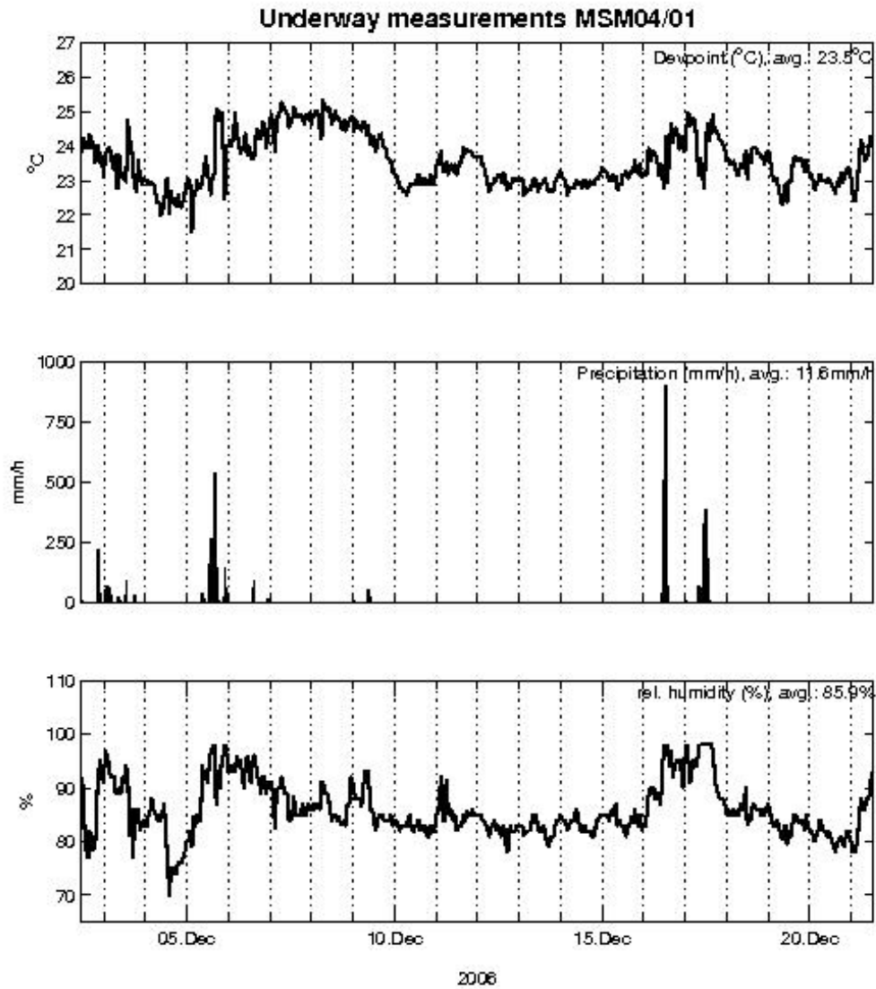
Fig. 1.8b : Time series from the ship's automated meteorological station, from top to bottom: dew-point, precipitation, relative humidity
