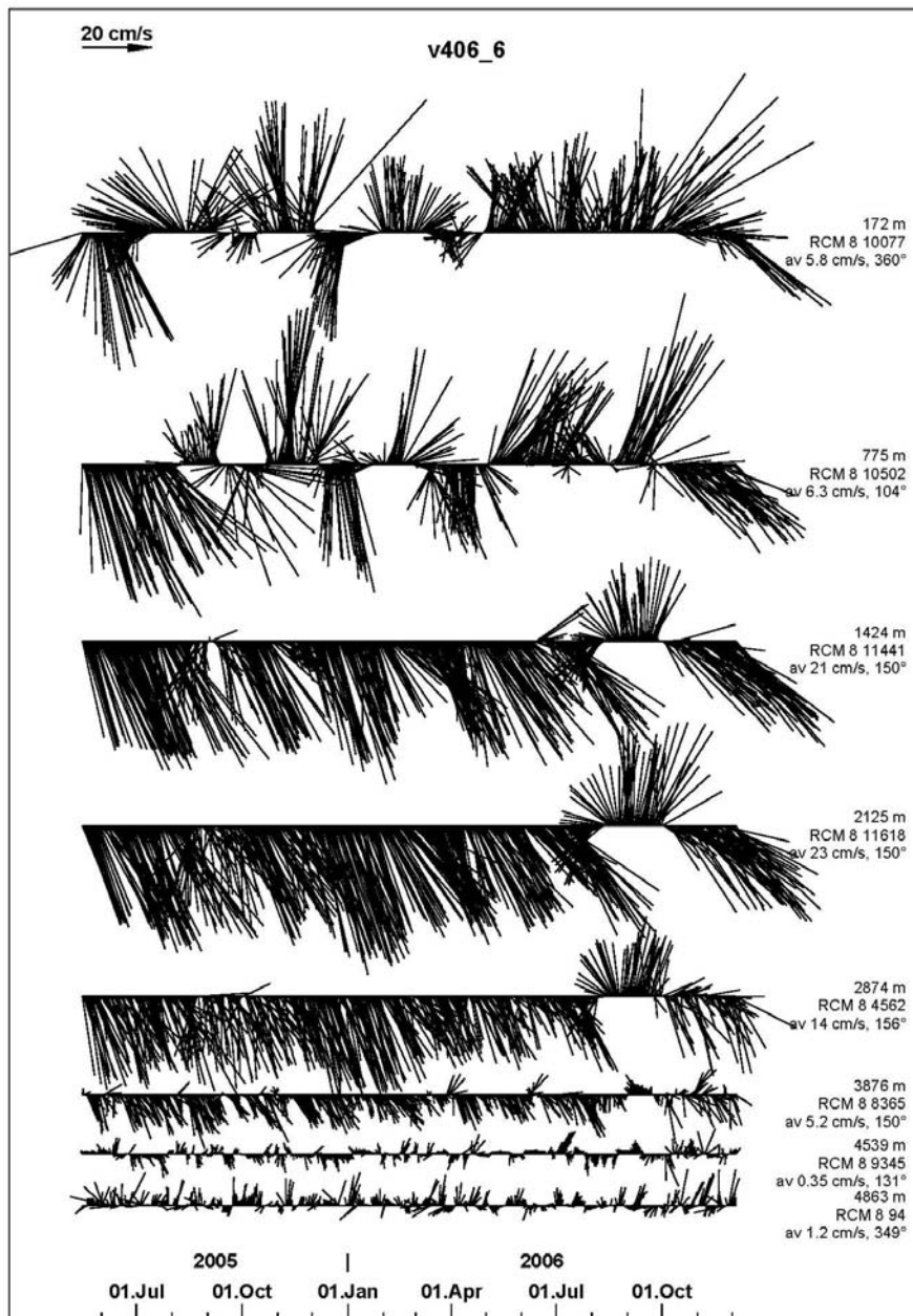
Fig. 1.4b: site M3, western geostrophic mooring V406-6, currents; up is north direction; depths and average currents indicated
