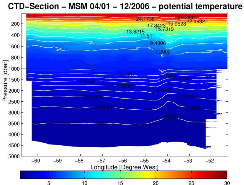
Fig. 1.2a: MSM04/1, potential temperature along 16° N.
