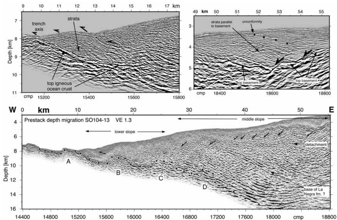
Figure 2.2.10: Pre-stack depth migration of Sonne 104 line 13 offshore Antofagasta (see Fig. 2.2.9 for location). Vertical exaggeration is 1.3. Note landward-dipping faults cutting the middle slope and soling out at a subhorizontal detachment at ~7 km depth. Black-filled circles mark the top of the subducting plate and letters indicate subducting horsts. Left close-up shows the well-stratified debris filling an incoming graben and forming the frontal prism. Right close-up shows the top of basement and overlying sediment cut and extended by normal faults. cmp: common mid point gather. (Ranero et al., in press, a)
