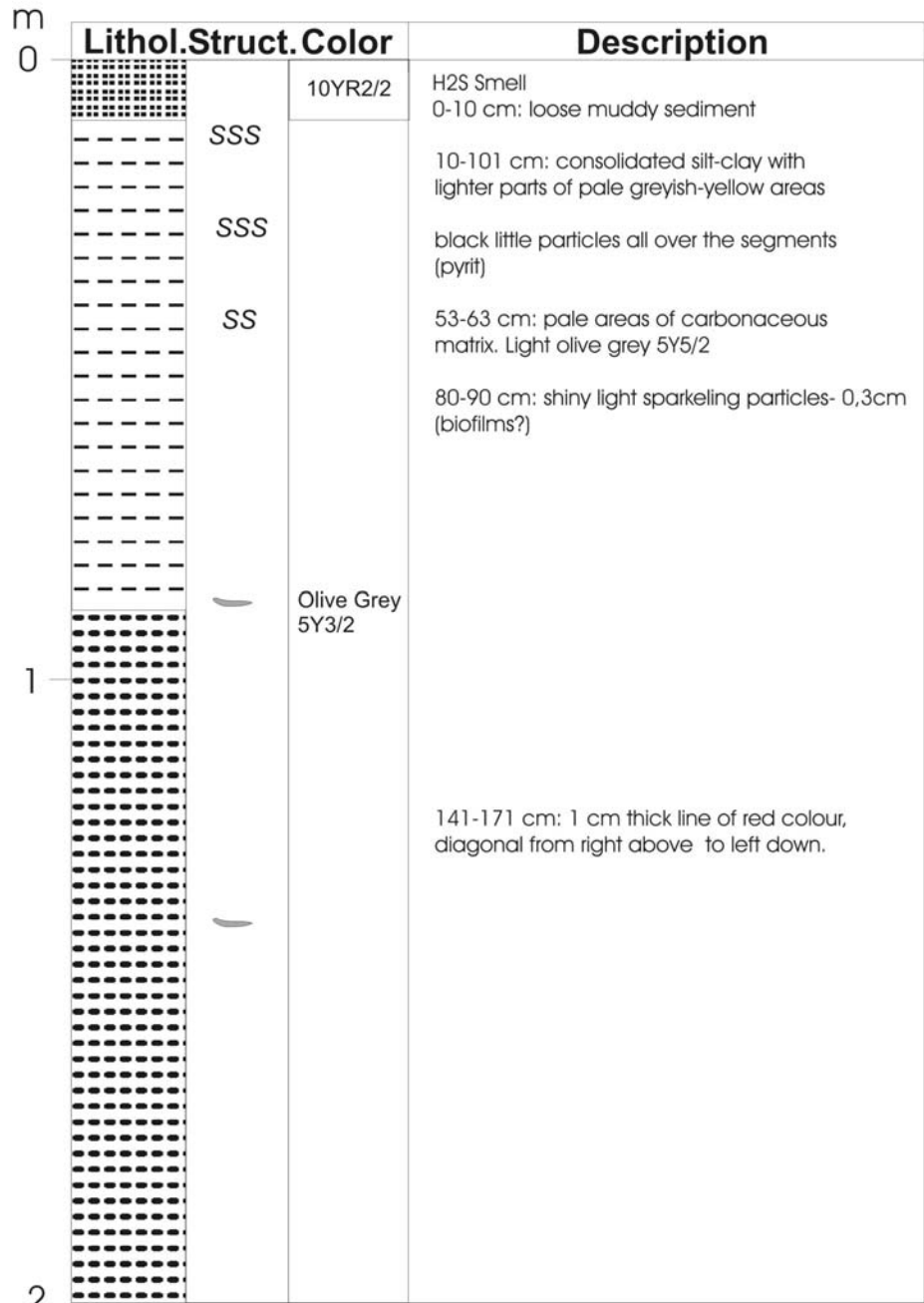
Figure 7.5.9: Core description Station M67-1/ 18/ 0-201 cm
