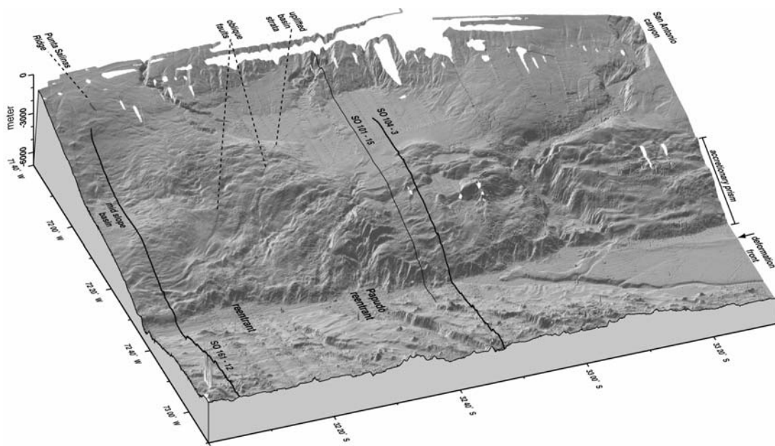
Figure 2.2.8: Perspective view from 290° azimuth and 38° elevation of shaded-relief bathymetry illuminated from 45°N. The data shows the area where the crest of the Juan Fernández Ridge has recently begun subducting. Note the deformed accretionary prism seawards of the Valparaíso Basin and the undisturbed accretionary prism south of the San Antonio canyon, where the trench is flooded with turbidites. (Ranero et al., in press, a)
